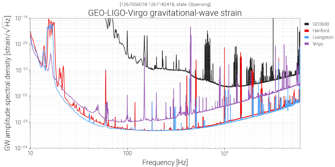
Figure 1: This plot represents the median noise of each interferometer measured over the course of the day. The measured output of each interferometer, calibrated to units of gravitational wave strain, is shown as a function of frequency. Since the amplitude of a gravitational wave signal changes with frequency, the shape of this curve determines each detector’s sensitivity to incoming gravitational waves. This plot is often referred to as the “noise curve”. (Plot from the Gravitational Wave Open Science Center summary status page, https://www.gw-openscience.org/detector_status/day/20200301/ )
